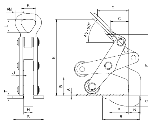
Model TWH s valčekmi
